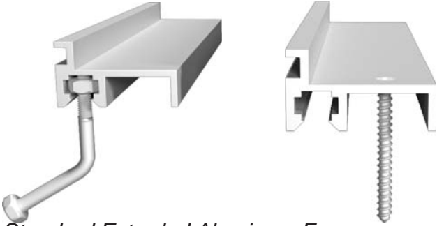
Standard Extruded Aluminum Frame Available in cast-in and blockout installations
