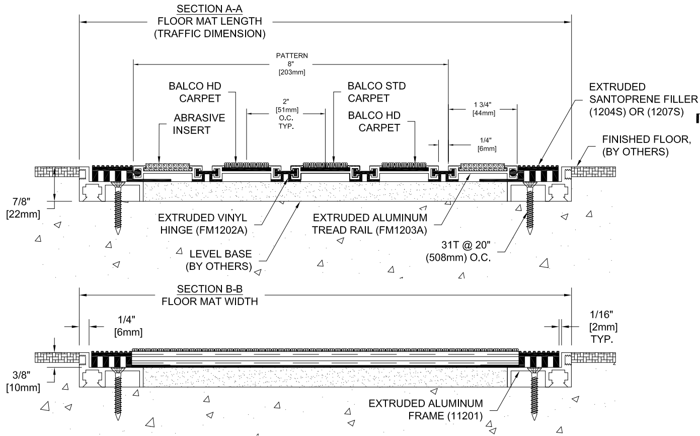
SECTION VIEW
