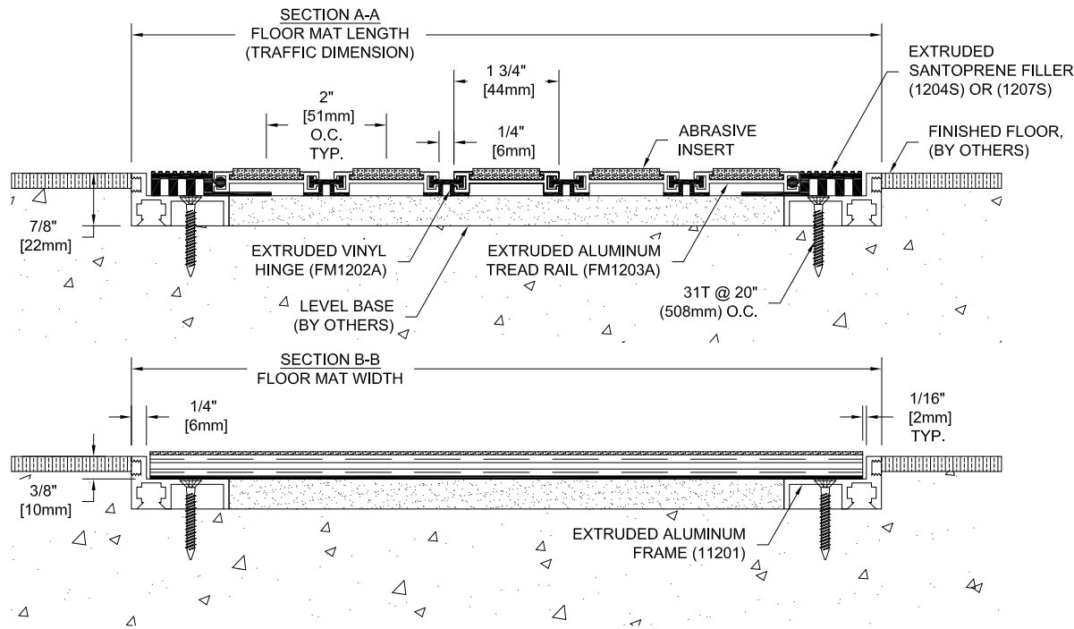
SECTION VIEW
